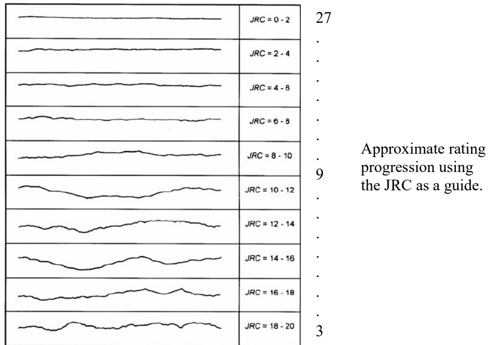
Figure 19. Joint Roughness Coefficient (JRC) guide, modified here as dimensionless. Low JRC values for macro roughness (large planar joints) joints would equate to a higher score. Rough, irregular joints (high JRC), both in macro and micro scale, score low.
