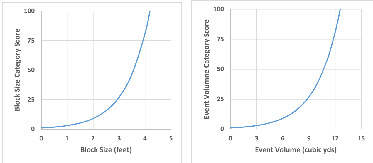
Figure 11. Chart pair illustrating the relationship between the block size and the category score and between the event volume and the category score. Note that the category score for block size maxes out for block sizes greater than 4 feet, while the category score for event volume maxes out for events over 12 cubic yards.
