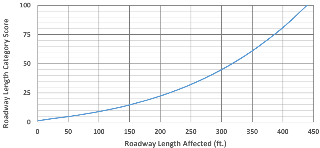
Figure 8. Chart illustrating the relationship between the length of roadway affected and the category score. The category score maxes out at an affected roadway length of about 440 feet.
